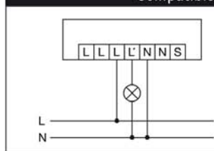
Installation standard
