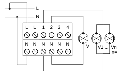
Figure 2: Wiring example: one valve per output and several valves per output.
