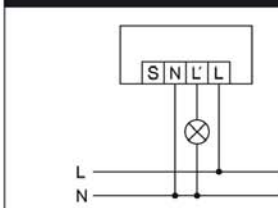
Installation standard
